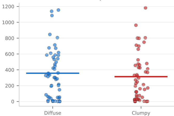
n_typing_bursts d=+0.10 p=0.631
