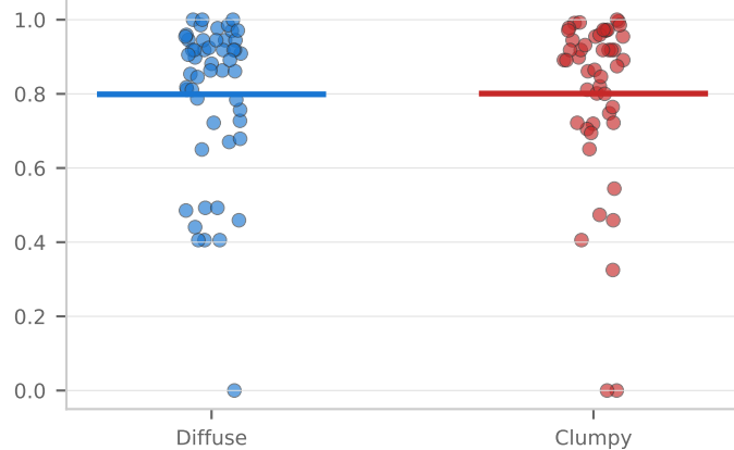
seq_time_entropy d=-0.01 p=0.964
