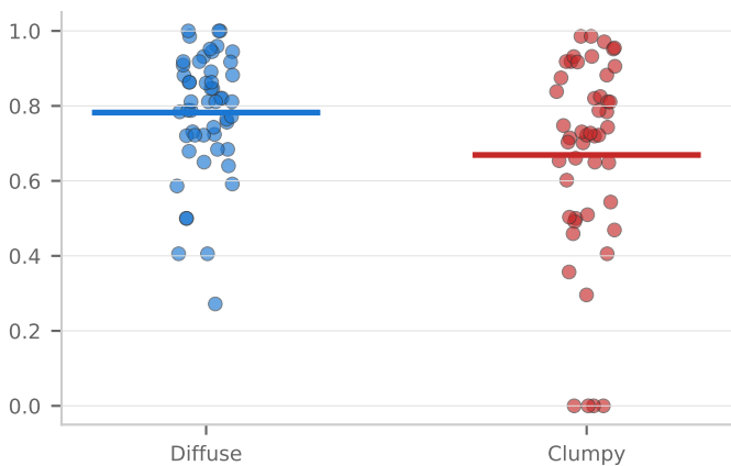
seq_typing_entropy d=+0.52 p=0.012
