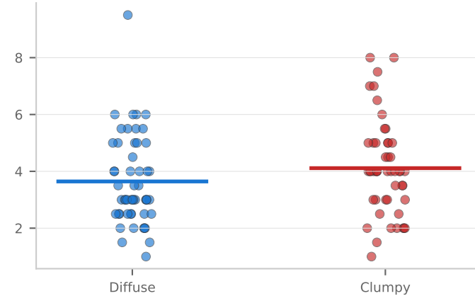
seq_topic_max_run d=-0.29 p=0.150
