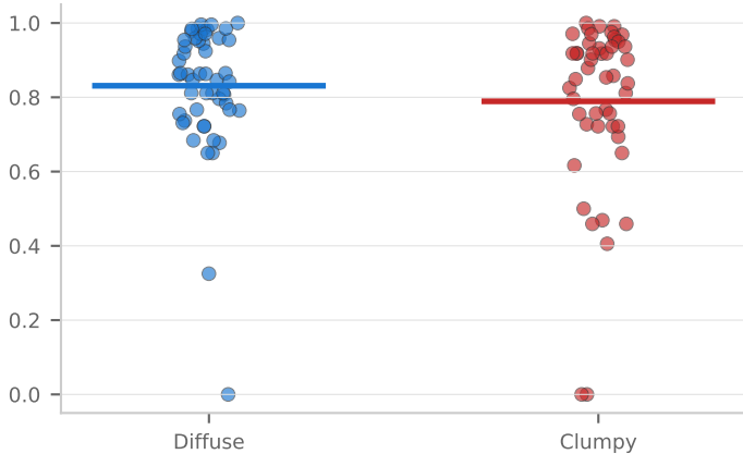
seq_topic_entropy d=+0.21 p=0.304
