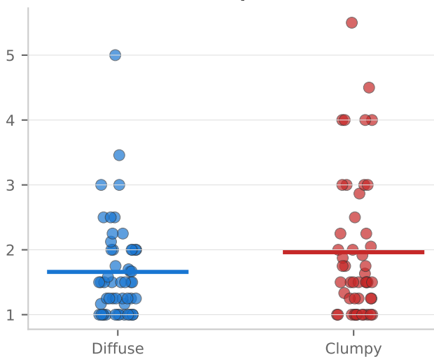
seq_topic_mean_run_exploit d=-0.32, p=0.110
