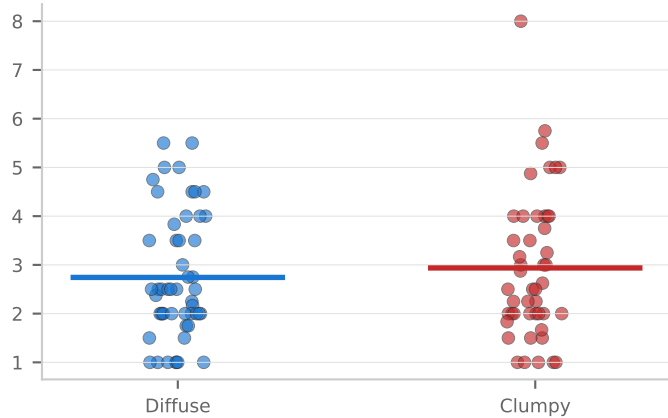
seq_topic_entropy d=+0.21 p=0.304
