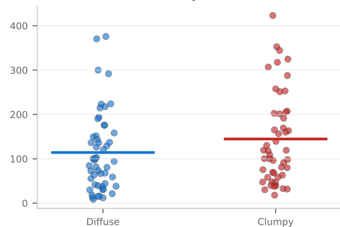
first_writing_time_s d=-0.32 p=0.115
