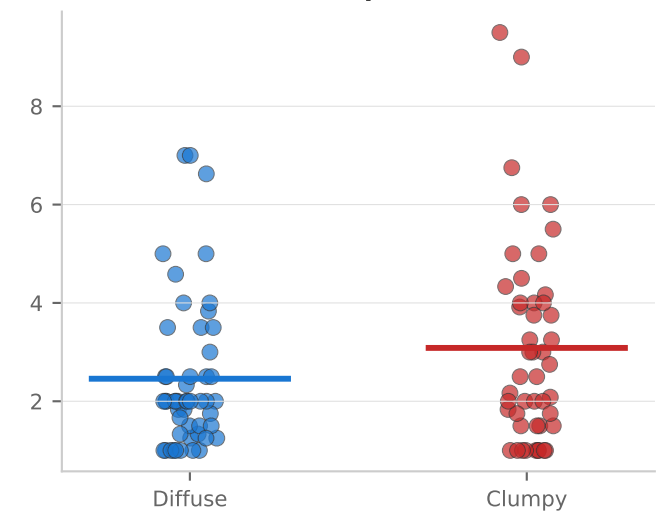
seq_time_mean_run_explore d=-0.35, p=0.091
