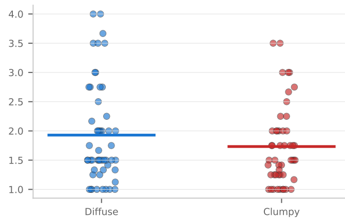
seq_time_mean_run_exploit d=+0.25 p=0.201
