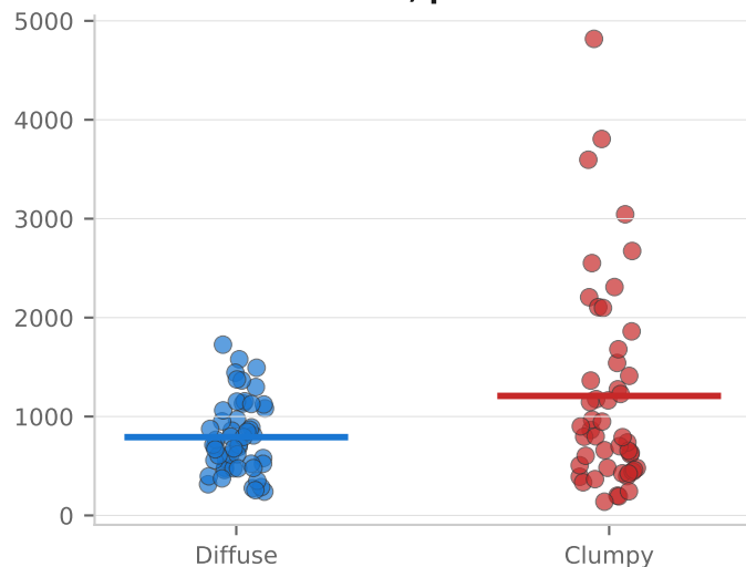
seq_typing_max_run d=-0.41, p=0.043
