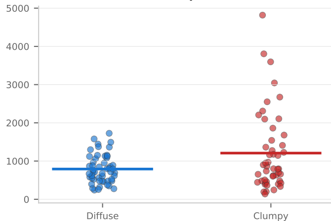
final_answer_length d=-0.54 p=0.010
