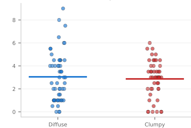
prop_pages_with_writing d=+0.05 p=0.790
