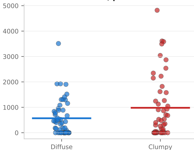
seq_topic_mean_run_exploit d=-0.32, p=0.110
