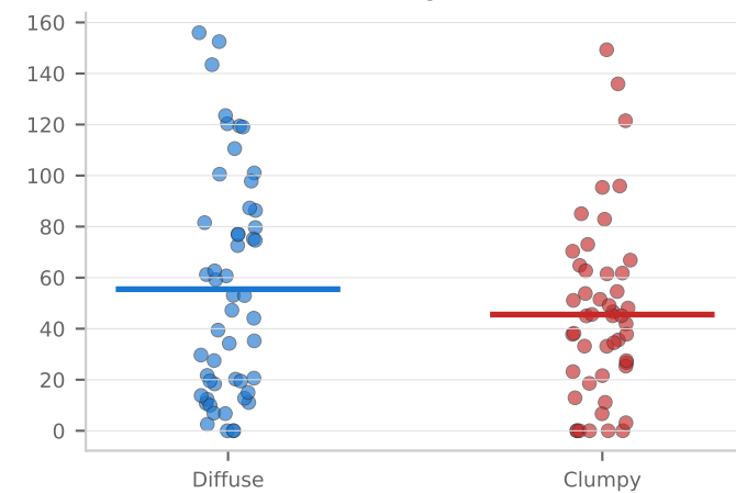
writing_gini d=-0.13 p=0.523
