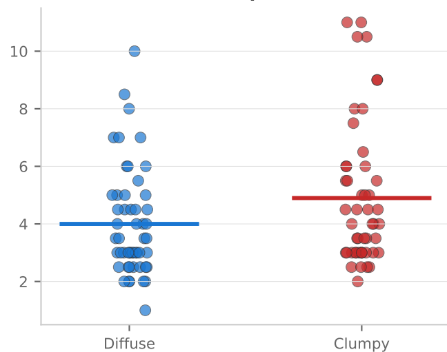
seq_typing_max_run d=-0.41, p=0.043
