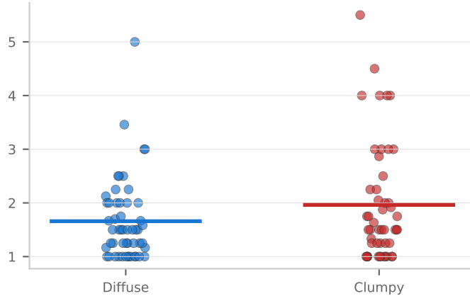
seq_topic_mean_run_exploit d=-0.32 p=0.110
