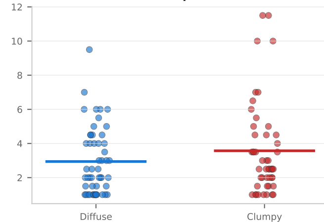
first_writing_page d=-0.27 p=0.187
