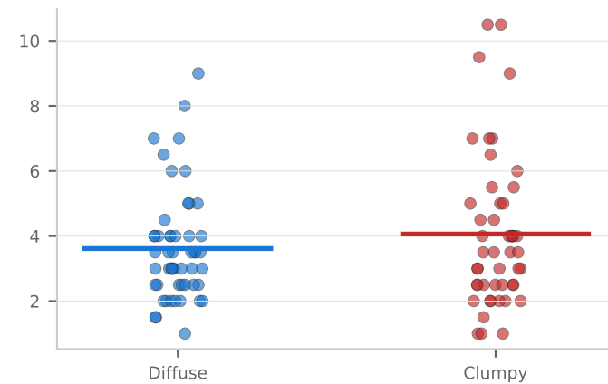
seq_time_max_run d=-0.22 p=0.278
