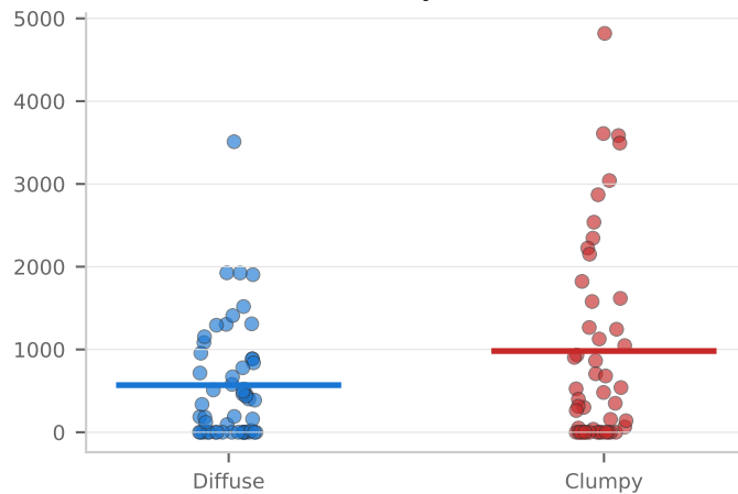
typing_duration_s d=+0.25 p=0.209
