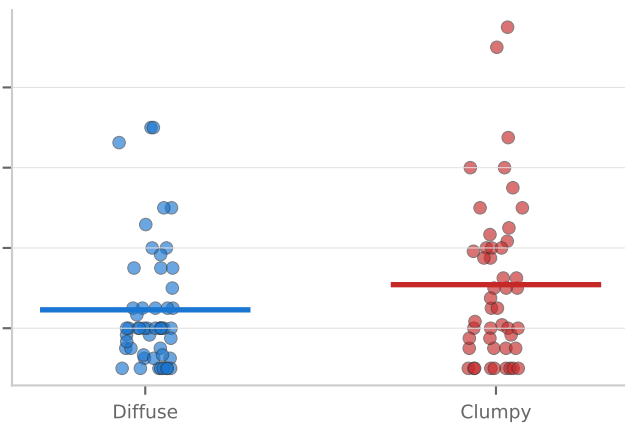
seq_time_entropy d=-0.01 p=0.964
