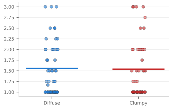
seq_typing_mean_run_exploit d=+0.03 p=0.884
