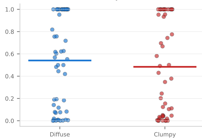
n_paste_events d=-0.29 p=0.148
