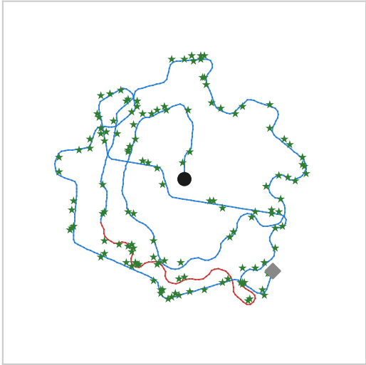
Trial 1 | Diffuse_1 | N=134
