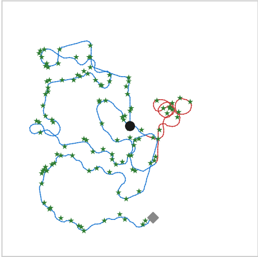
Trial 2 | Diffuse_4 | N=118
