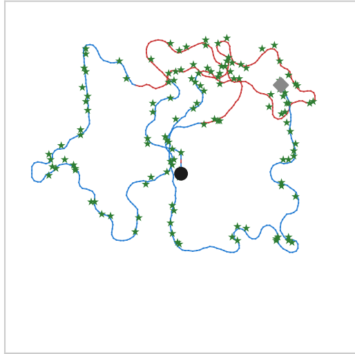
Trial 4 | Diffuse_4 | N=132
