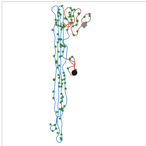
Trial 1 | Diffuse_5 | N=107
