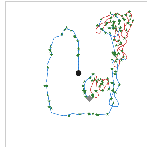
Trial 5 | Diffuse_5 | N=134
