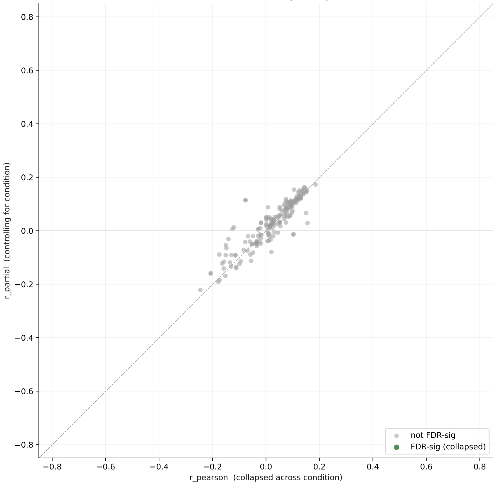
M78 Robustness: each correlation, collapsed vs partial-out condition
