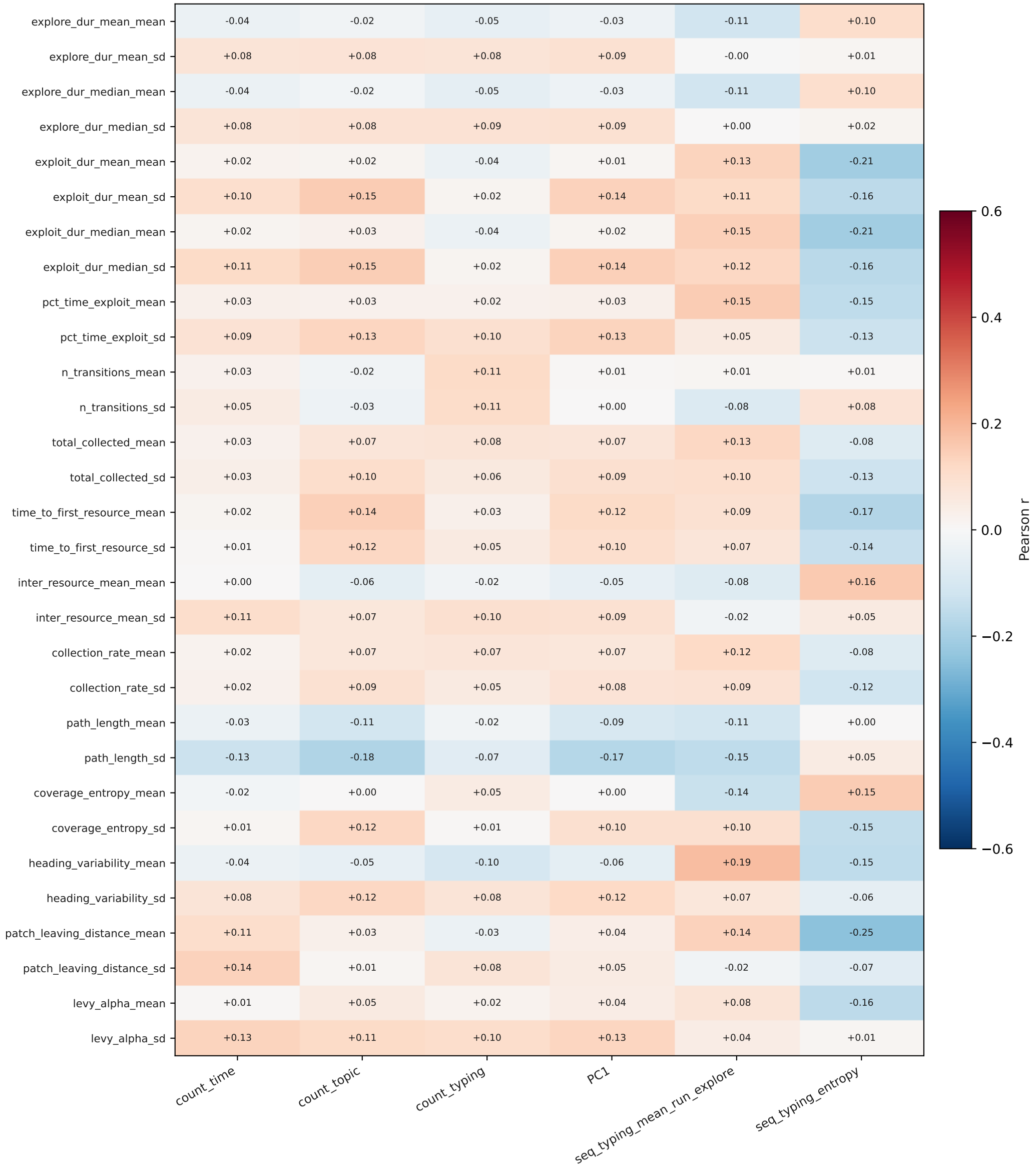
M78 Pearson r (Spatial 30 x Wiki 6 = 180) * = FDR-BH < 0.05
