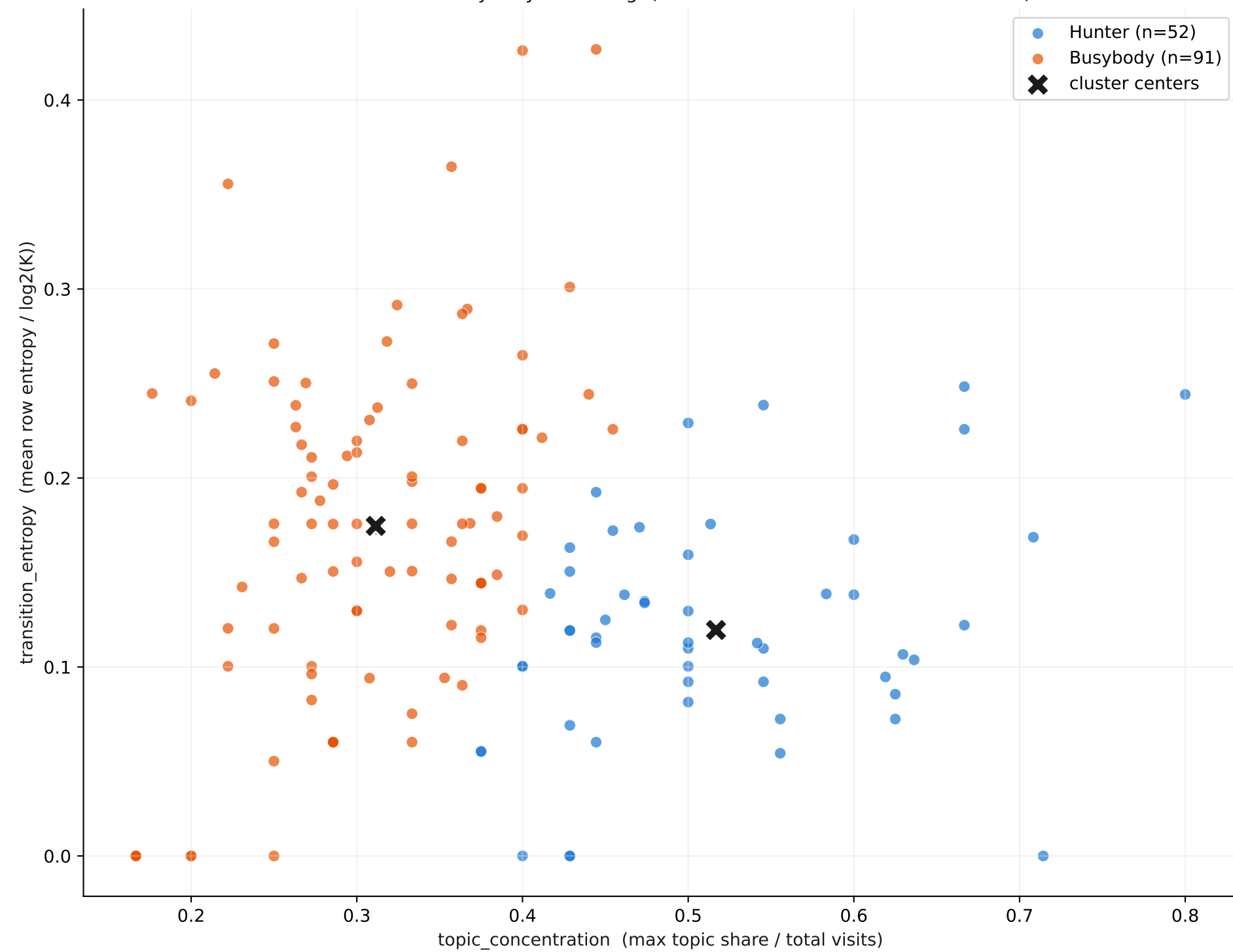
M80 Hunter vs Busybody clustering (KMeans k=2 on standardised features)
