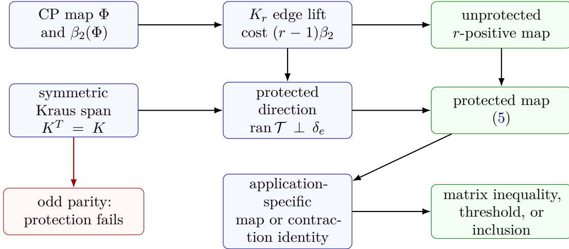
FIGURE 1. A diagnostic for applying the rank-two lifting theorem. The rank-two constant and even transpose parity are universal inputs. Concrete downstream formulae require a separate identity for the chosen map.
