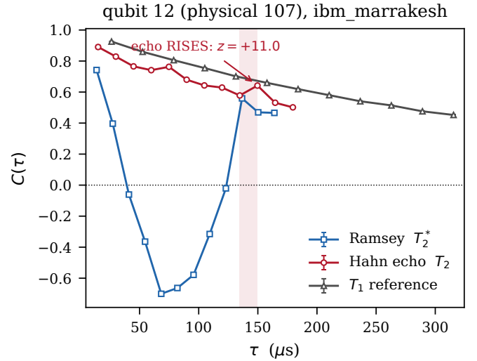
FIG. 3. The three arms on one qubit, with error bars. The Ramsey arm oscillates — a detuning of a few kHz, not a pathology of the envelope — while the echo arm decays and then rises in the shaded segment. The T_1 reference decays monotonically throughout. Normalisation is by the measured \tau = 0 point of each arm.
