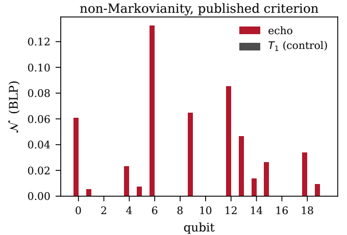
FIG. 5. The Breuer–Laine–Piilo witness \mathcal{N} per qubit: the echo arm against the T_1 control. A criterion taken from the non-Markovianity literature, computed on the same counts, singles out the same qubits as the representability test of Table XII.
