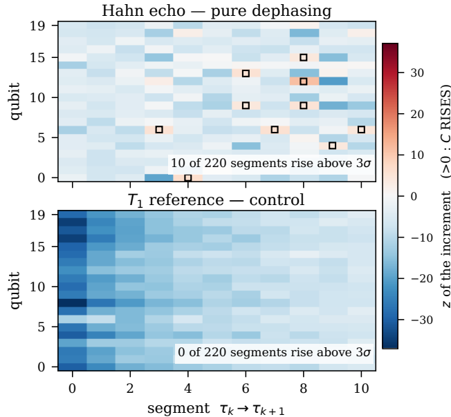
FIG. 4. Increment z between consecutive delays, qubit by qubit. Black squares mark rises above 3\sigma . Top: the echo arm. Bottom: the T_1 control, on the same scale. The refutation is read off the raw counts: no model is fitted anywhere in this figure.
