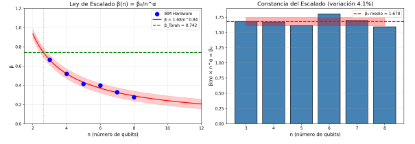
FIG. 8. Scaling law \beta(n) = \beta_0/n^\xi for GHZ states on IBM ibm_fez . R^2 = 0.987 .
