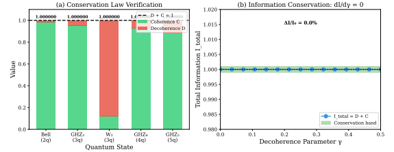
FIG. 2. Conservation law D + C = 1 verification across five quantum states on IBM ibm_torino . All states show exact conservation to numerical precision, confirming the topological invariance of total information.
