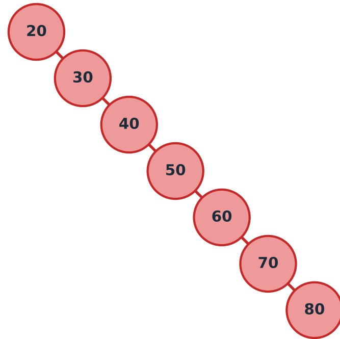
(b) Insertions triées — h = n - 1 = 6, \mathcal{O}(n)
