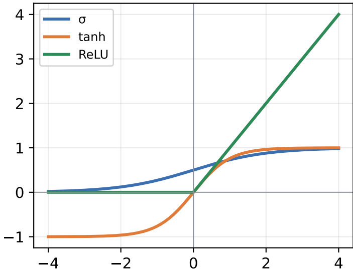
Activations
