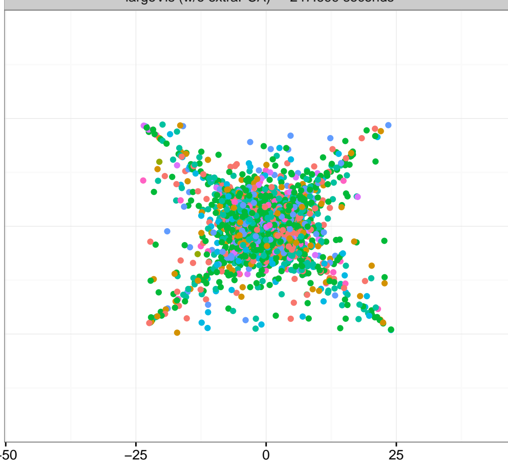
largeVis (w/o extraPCA) – 247.699 seconds
