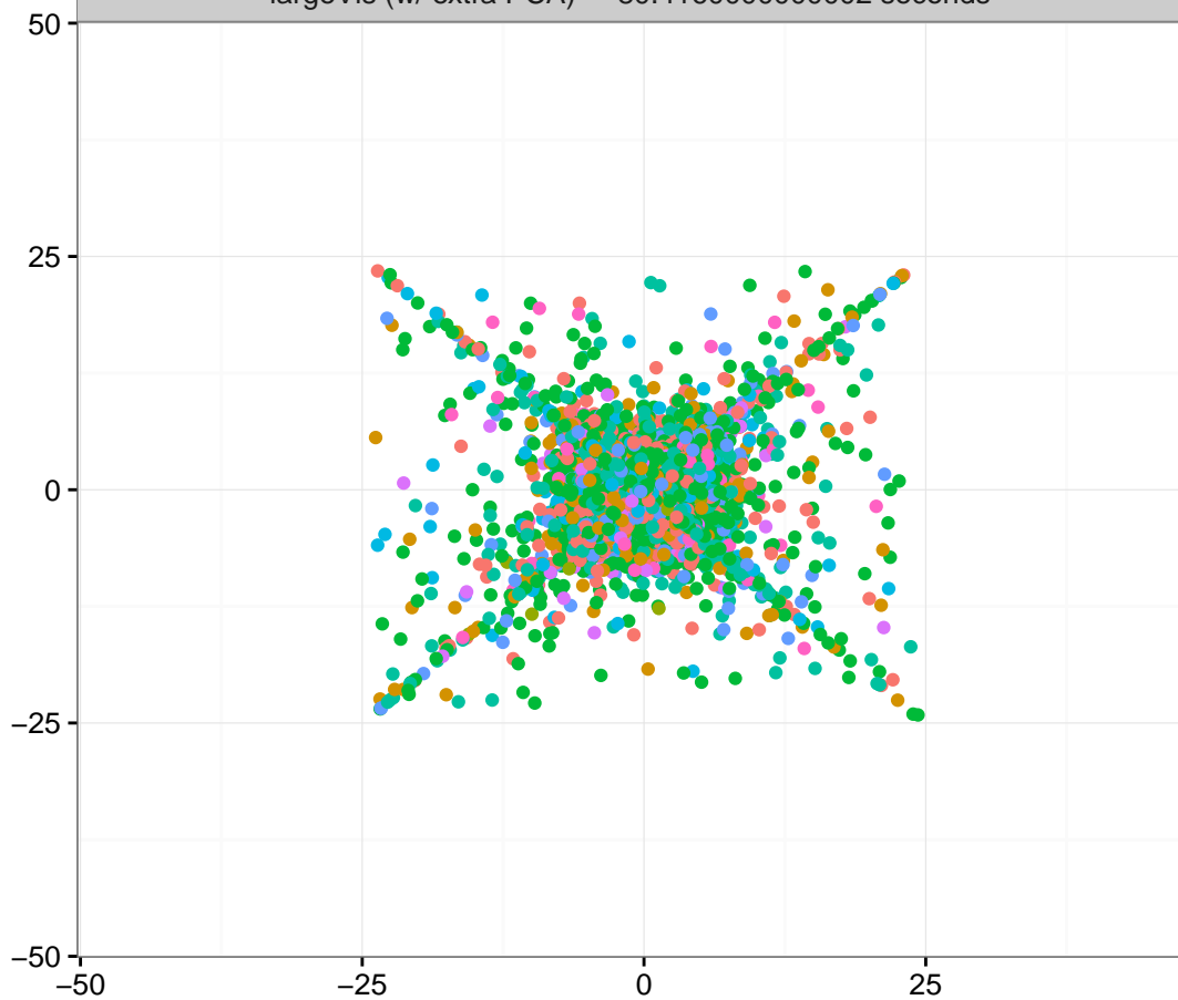
largeVis (w/ extra PCA) – 80.4160000000002 seconds
