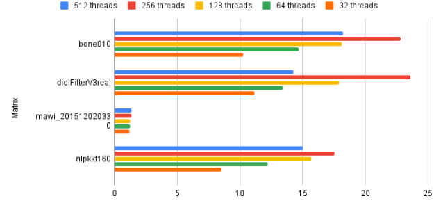
GFLOP/s changing threads per block
