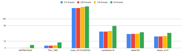
Fig. 10. Execution time (ms) for the warp level kernel (lower is better)
