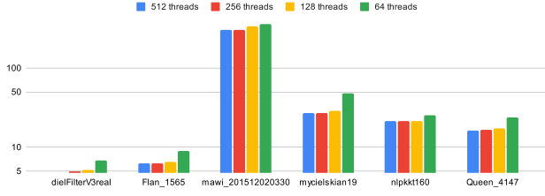
Fig. 11. Execution time (ms) for the warp level kernel with unroll (lower is better)
