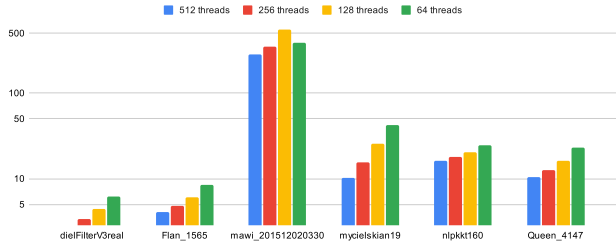
Fig. 12. Execution time (ms) for the share memory kernel (lower is better)
