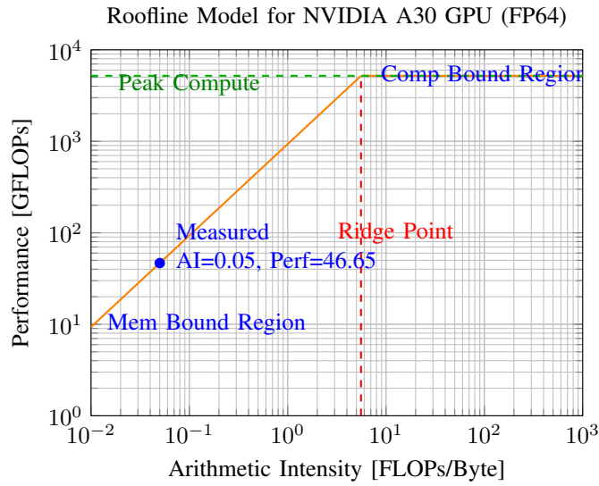
Fig. 5. Roofline Model For SpMV On NVIDIA A30
