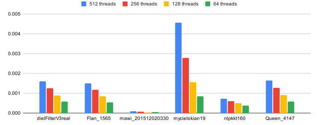
Fig. 15. Average GB/s developed by the share memory kernel (higher is better)
