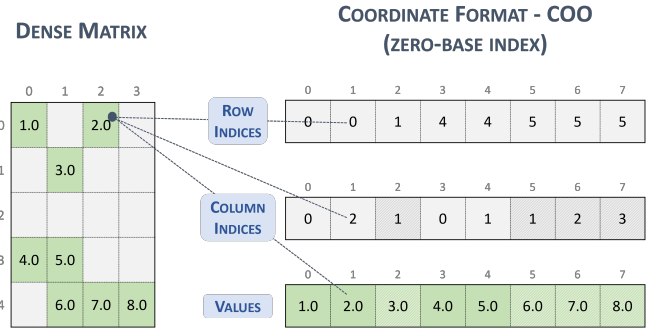
Fig. 1. Encoding of a matrix in COO format
