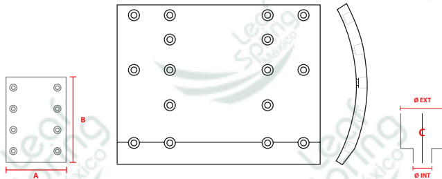
NO. PARTE FMSI HIN5001626R500
