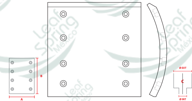
NO. PARTE FMSI / FAW JK6 2417 GNC
