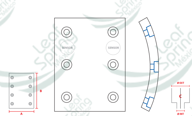
NO. PARTE FMSI FAW1607 F
