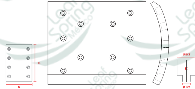
NO. PARTE FMSI / FAW 2412D
