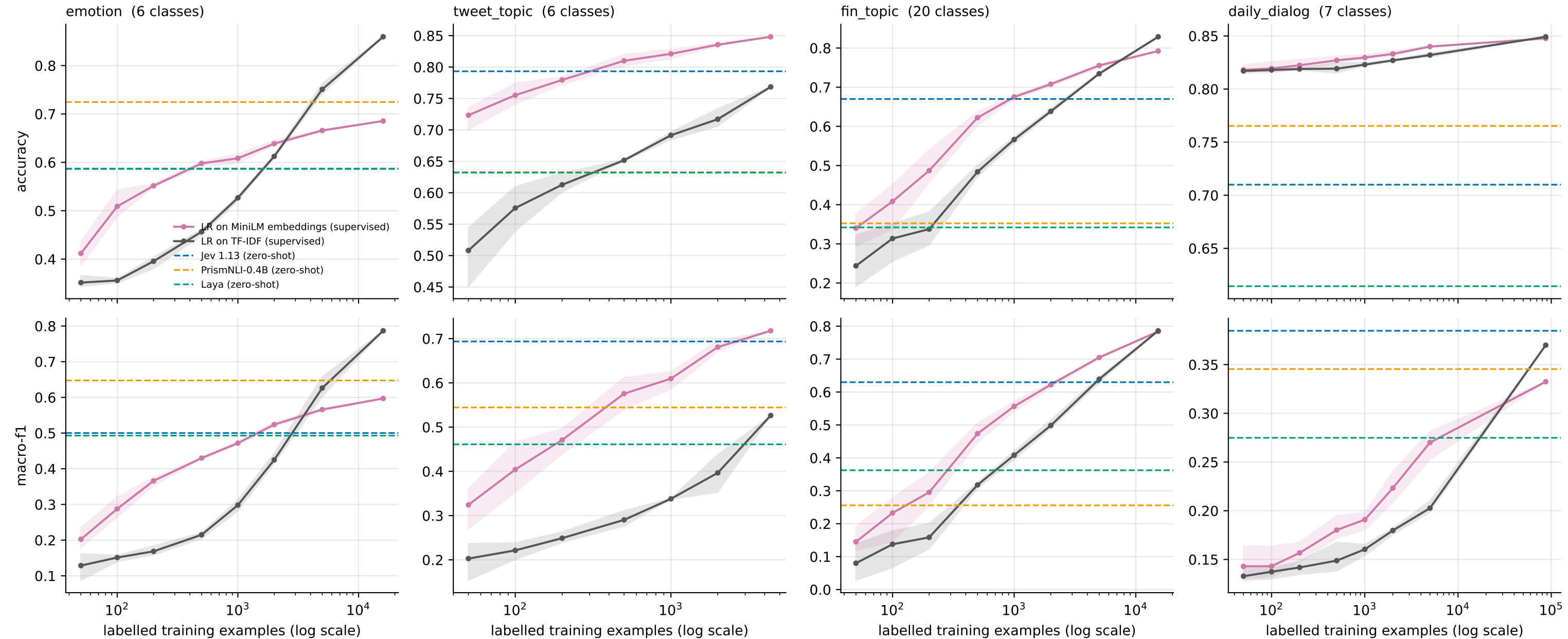
How many labels does a simple supervised model need to match the best zero-shot system? (mean of 3 seeds, band = min-max)
