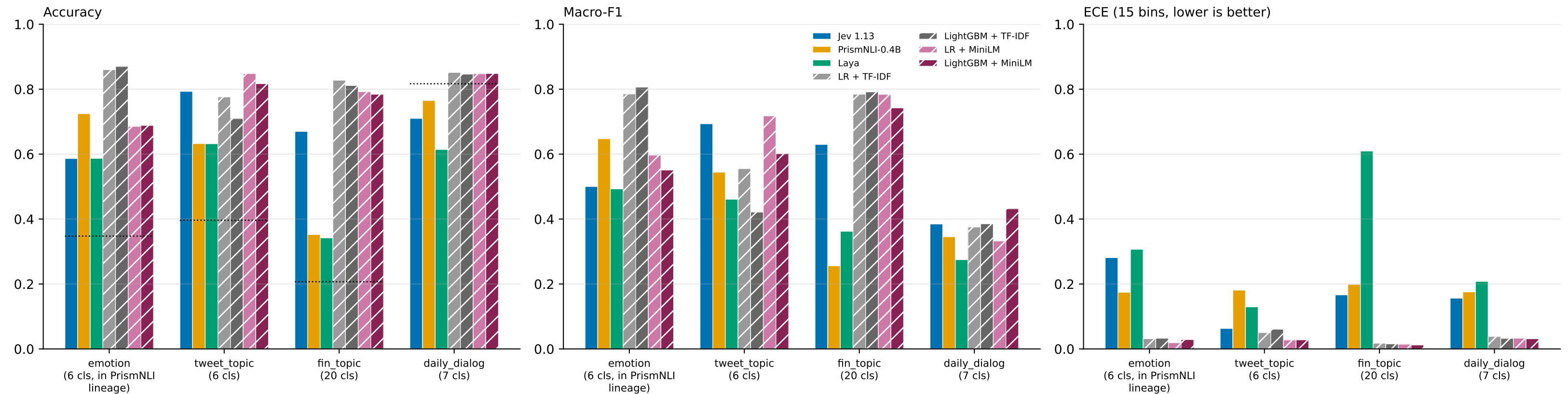
Zero-shot systems (solid) vs supervised models trained on each dataset's own labels (hatched), same evaluation rows
