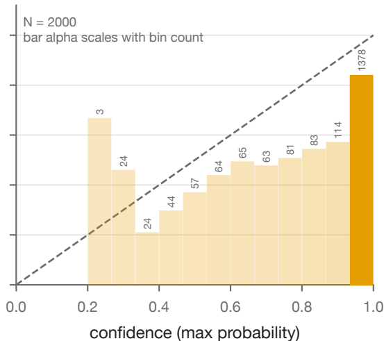
PrismNLI-0.4B (ECE = 0.174)
