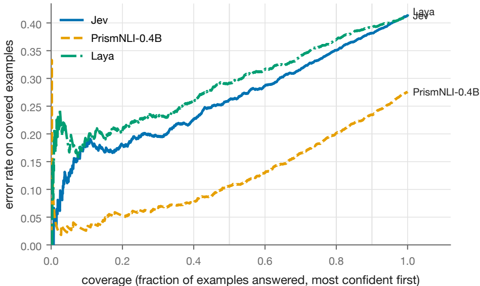
Risk-coverage curve
