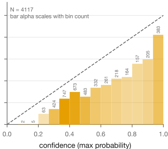
PrismNLI-0.4B (ECE = 0.199)
