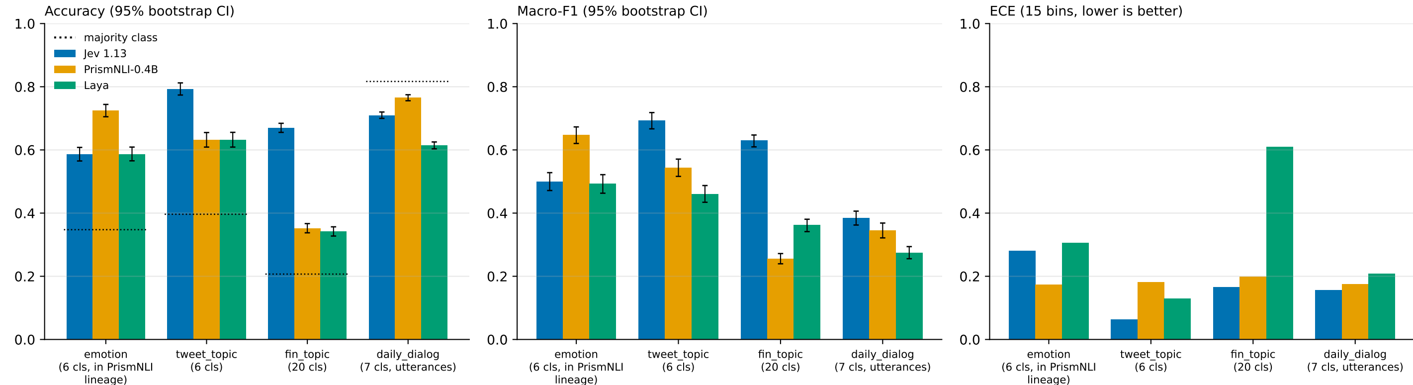
Zero-shot results across datasets (plain variant). Only dair-ai/emotion is in PrismNLI's training lineage.
