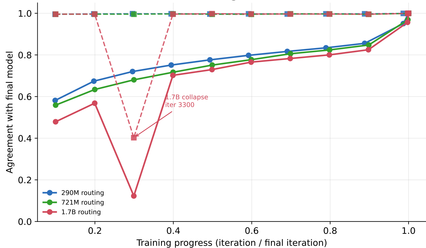
Volume (dashed) above routing (solid) at 290M / 721M / 1.7B
