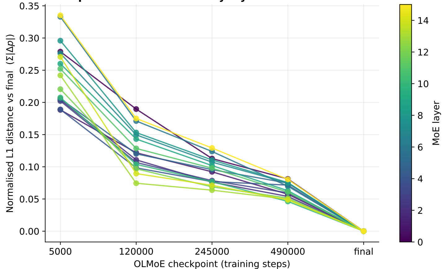
Expert-volume distance by layer in OLMoE-1B-7B
