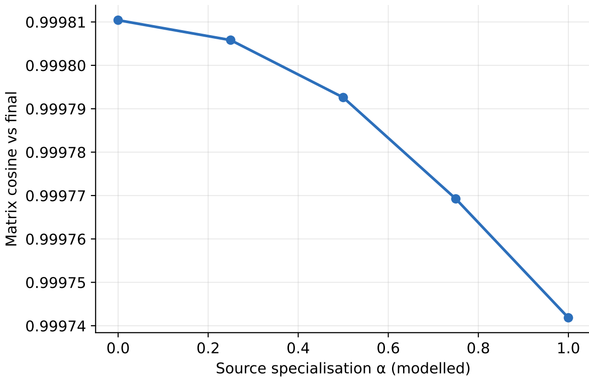
Matrix cosine vs \alpha (FLAME-MoE-290M)
