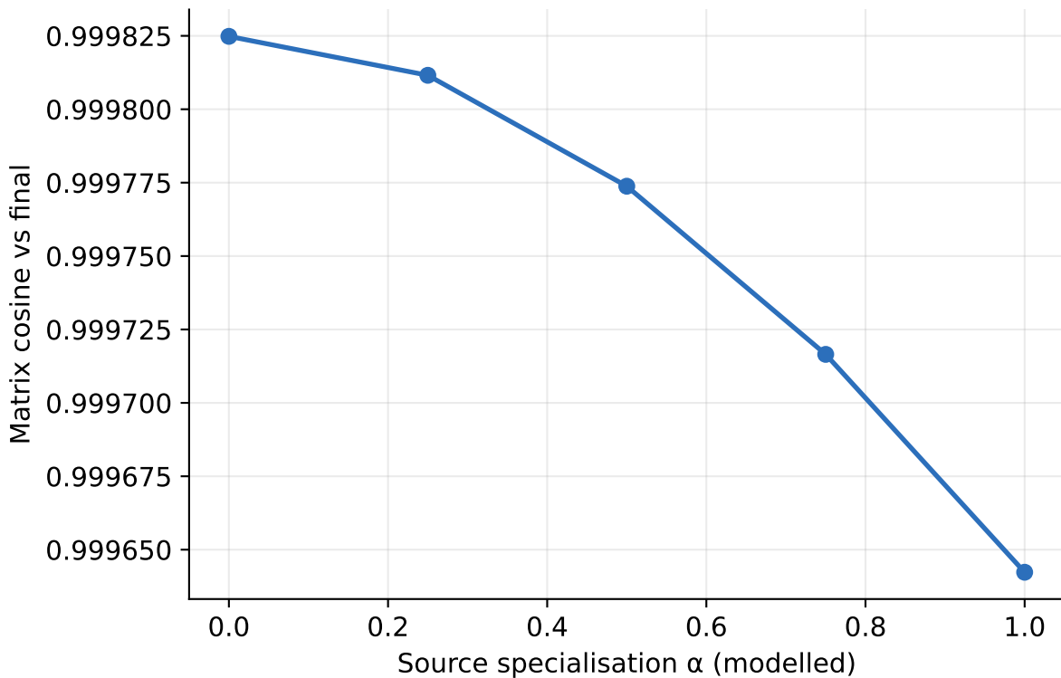
Matrix cosine vs \alpha (OLMoE-1B-7B)
