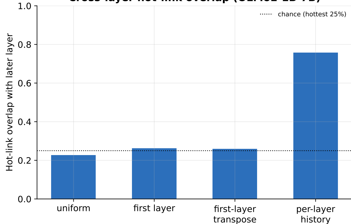
Cross-layer hot-link overlap (OLMoE-1B-7B)
