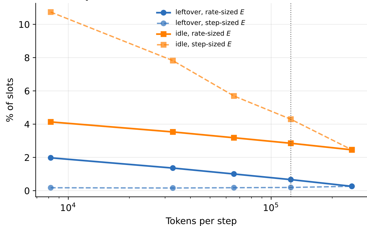
Per-step leftover of a frozen P95 (FLAME-MoE-290M)
