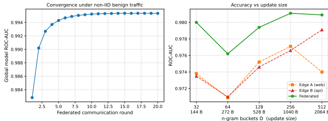
Fig. 3. Left: convergence of the global model. Right: accuracy against synchronisation payload size as the n -gram dimension D varies. The federated model balances detection across domains at every D .
