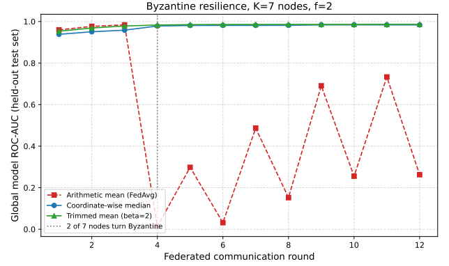
Fig. 4. Measured resilience to model poisoning. From round 4, two of seven nodes upload sign-flipped, 12\times amplified weights. Mean aggregation collapses; median and trimmed mean absorb the attack.
