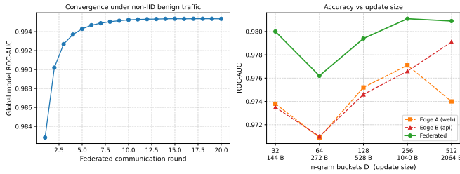
Fig. 3. Left: convergence of the global model. Right: accuracy against synchronisation payload size as the n -gram dimension D varies. The federated model balances detection across domains at every D .
