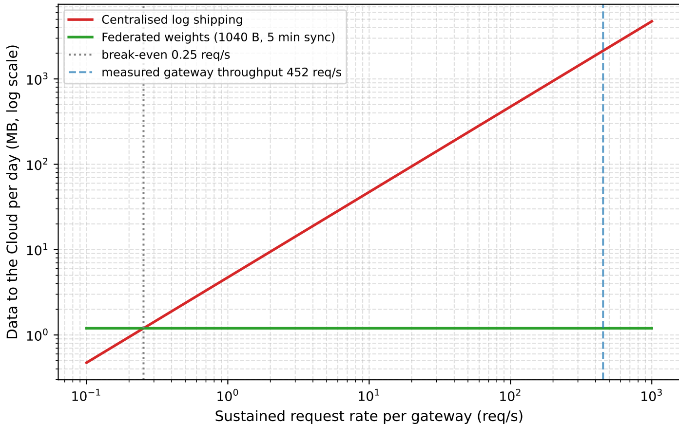
Bandwidth scaling: federated cost is independent of traffic
