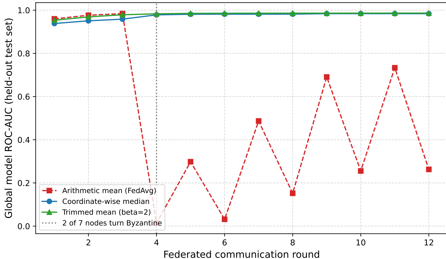
Byzantine resilience, K=7 nodes, f=2
