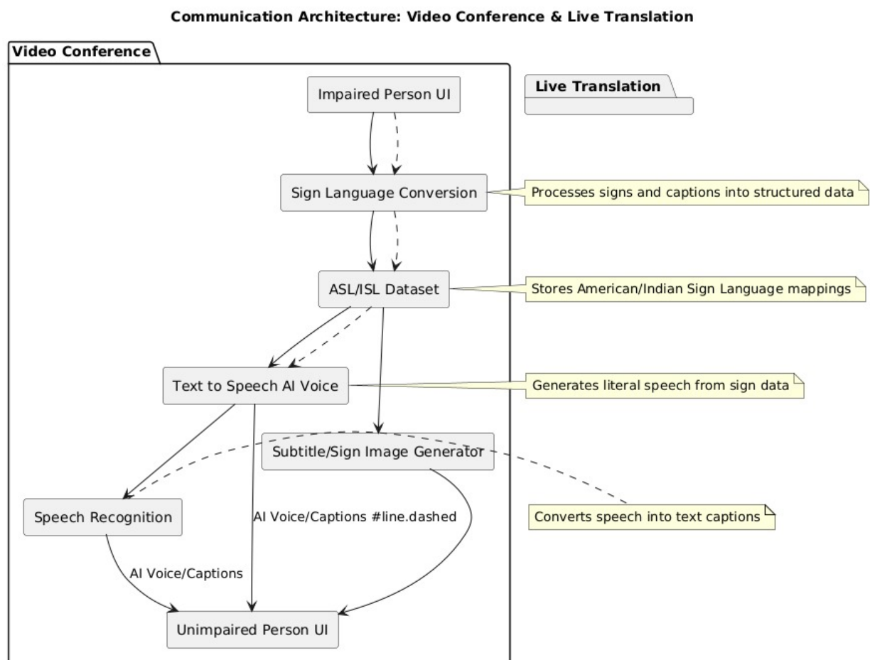
Figure 3.2: Architecture Diagram
