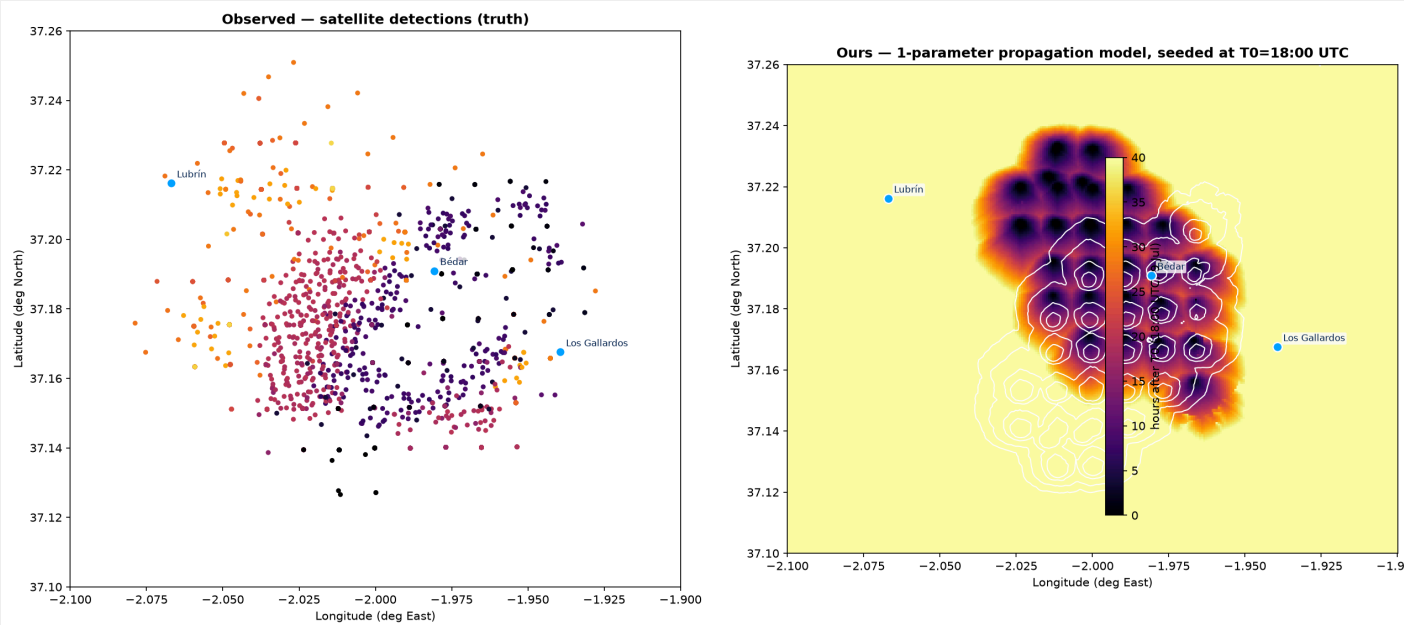
Left: real detections. Right: our model ( R_0=0.010 , wind 19 km/h toward 12°, WorldCover fuel, DEM slope) seeded from the detections before T0. Area matches within ~7% (6,191 vs 5,767 ha) but arrival-time MAE is 23 h — the mechanism works, the timing does not.
