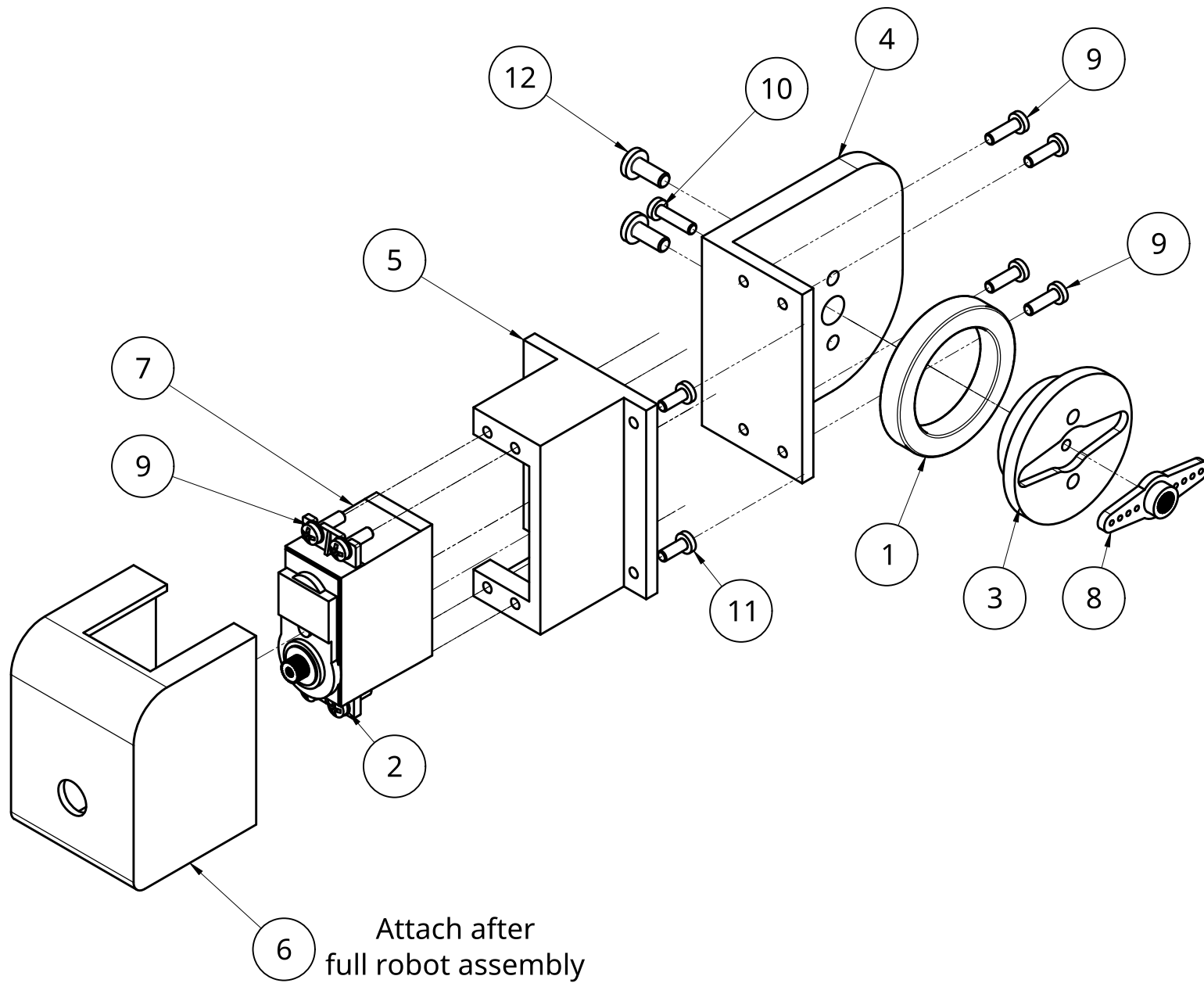
LINK 5 EXPLODED VIEW
