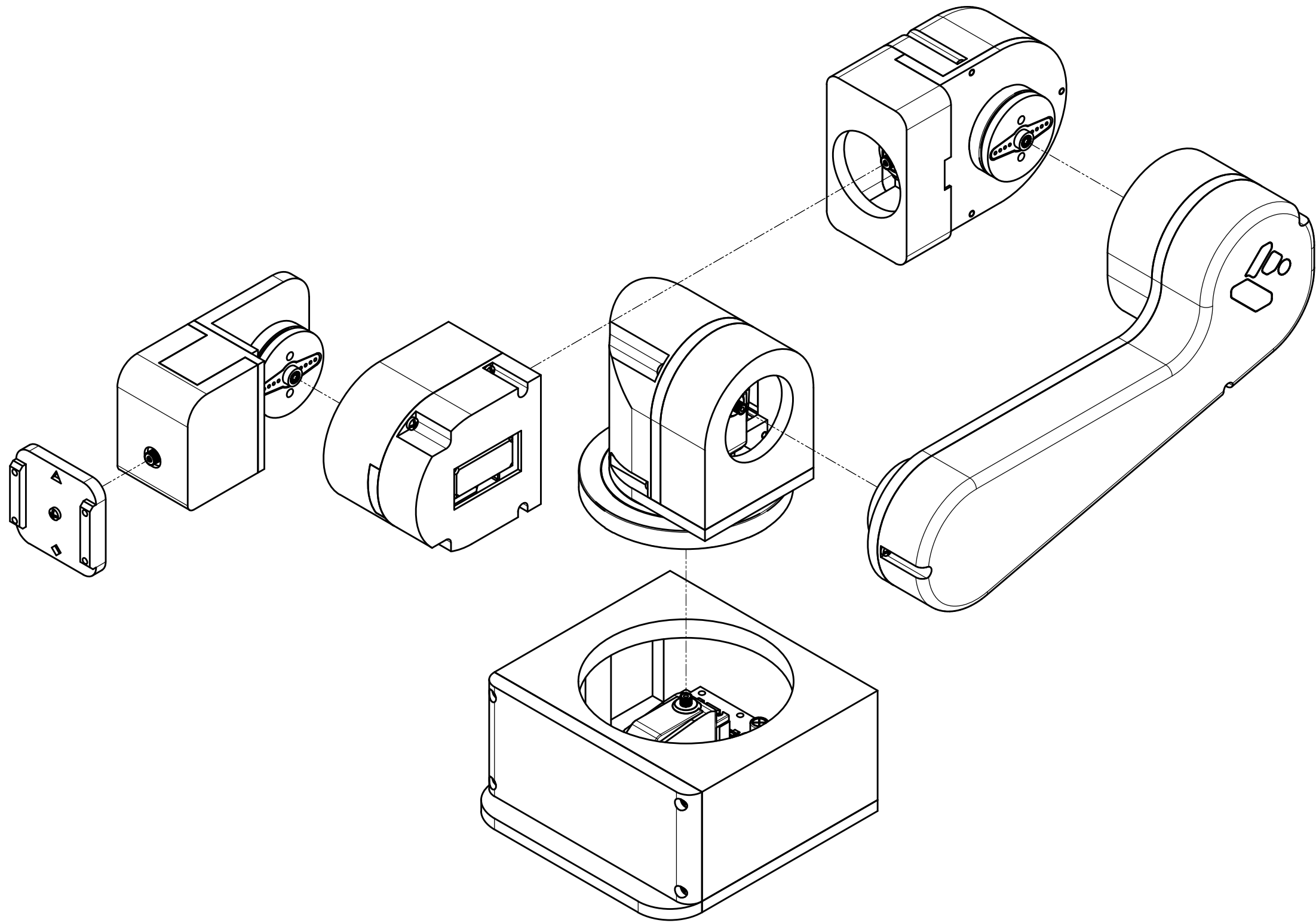
MORRIS V2 EXPLODED VIEW
