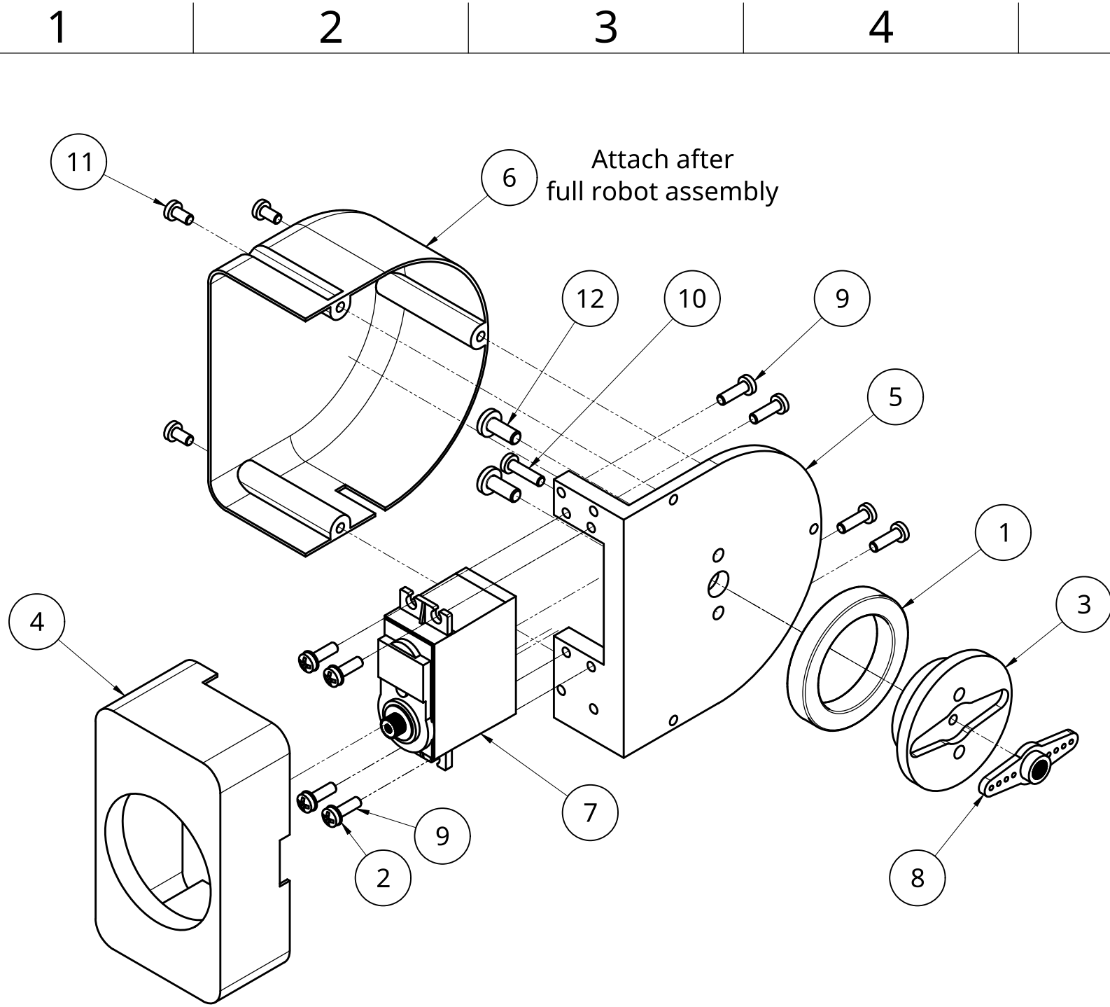
LINK 3 EXPLODED VIEW
