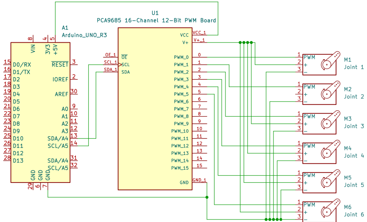
Figure 4: Schematic of the basic Mv2 electronics.
