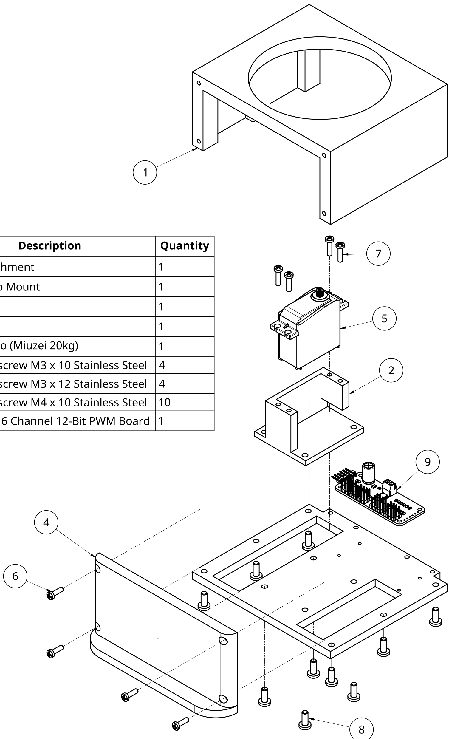
BASE EXPLODED VIEW
