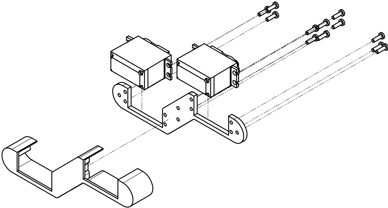
EXPLODED ISOMETRIC 1:2
