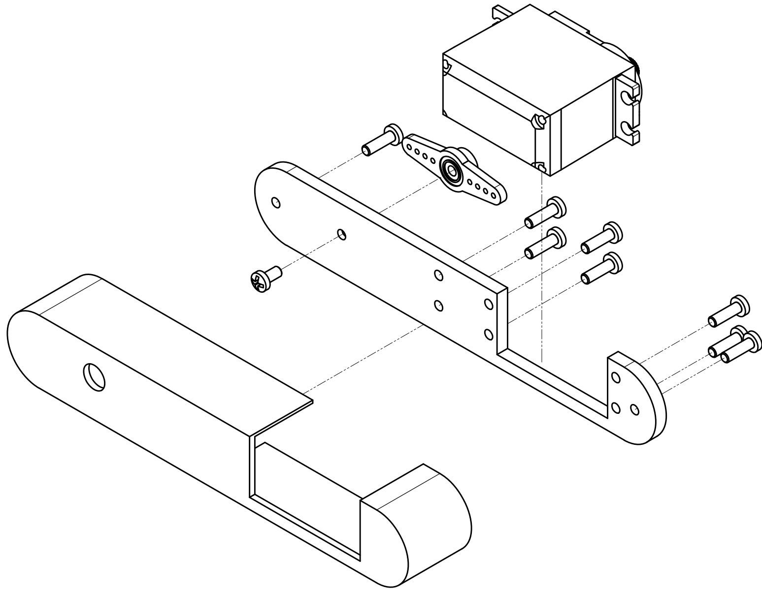
EXPLODED ISOMETRIC
