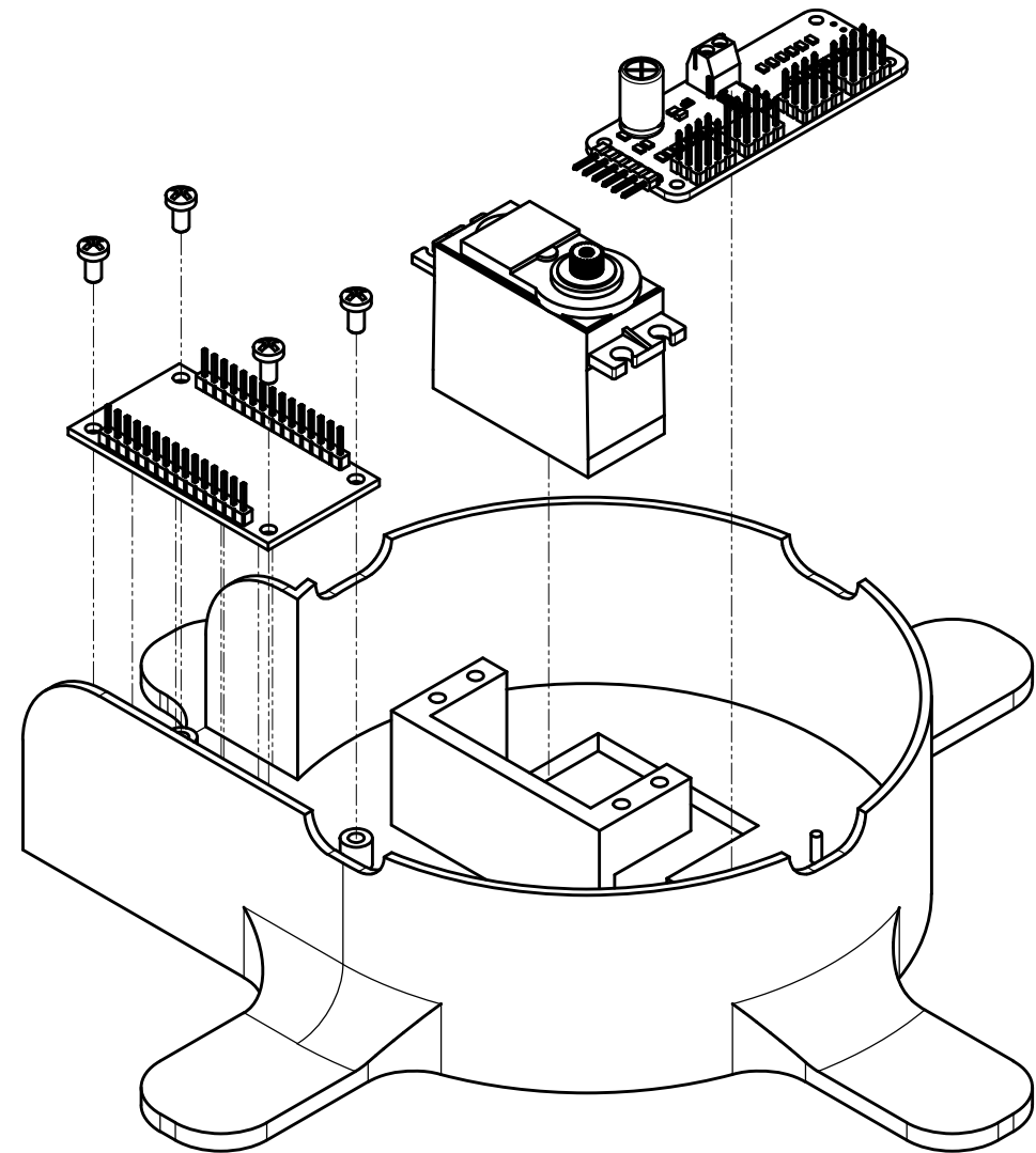
EXPLODED ISOMETRIC 1:1.5
