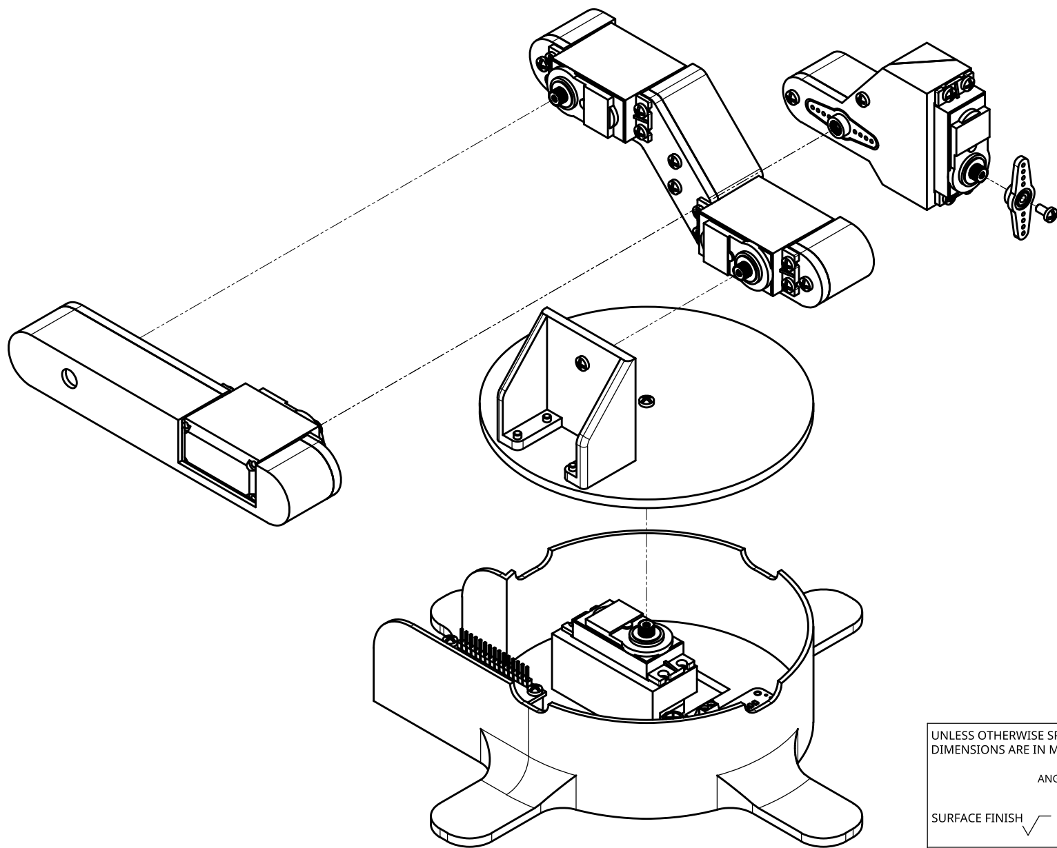
EXPLODED ISOMETRIC 1:2
