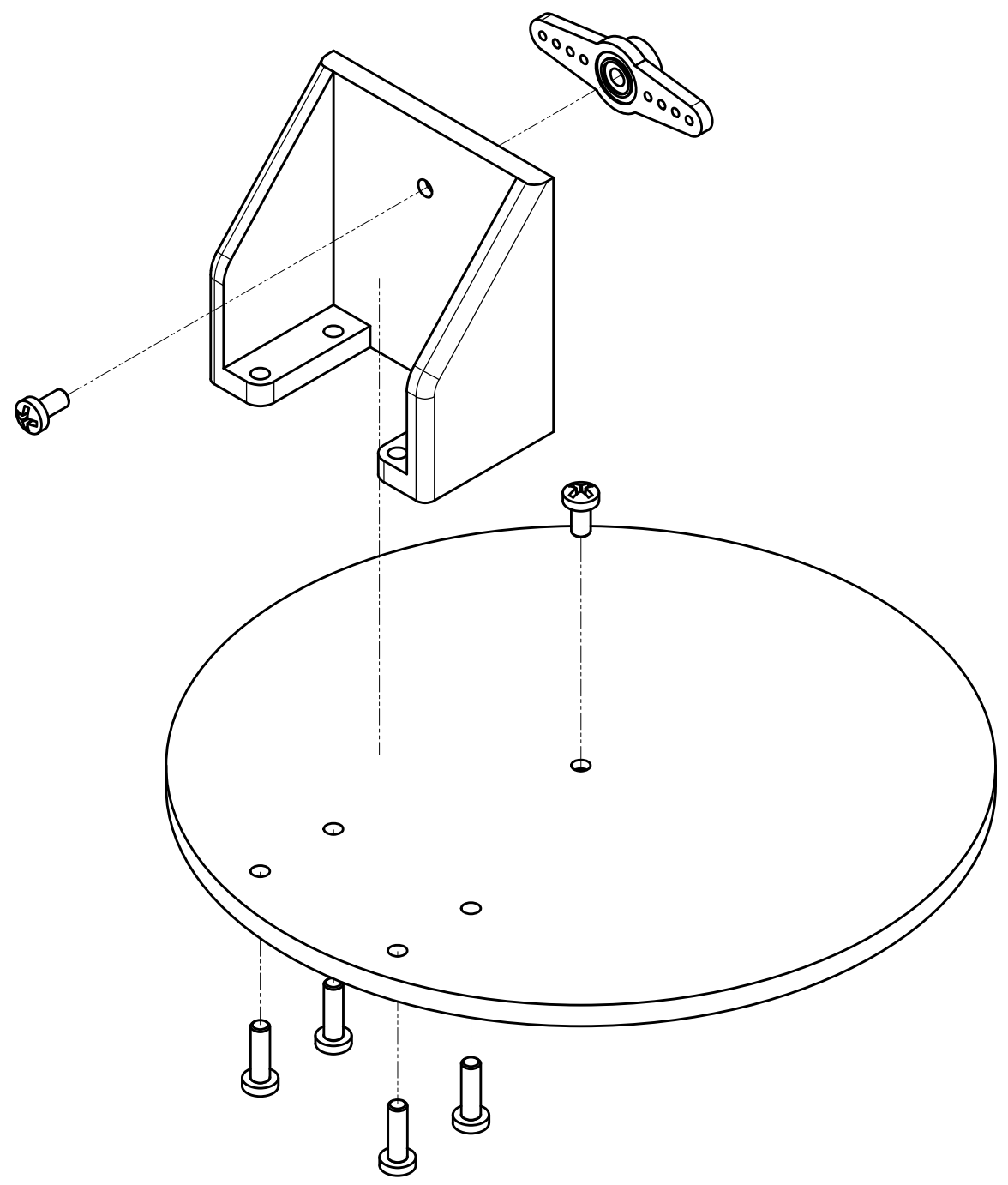
EXPLODED ISOMETRIC
