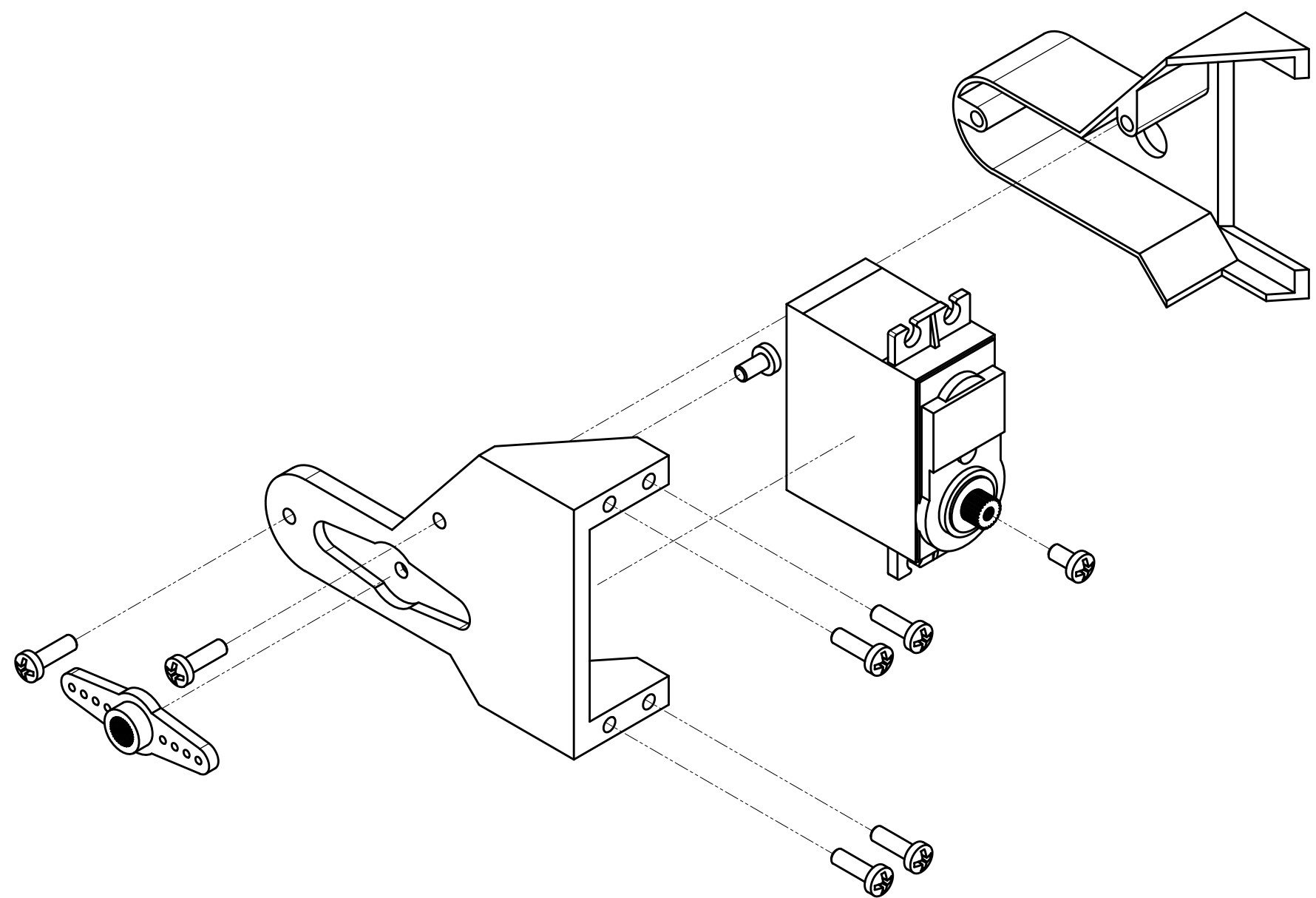
EXPLODED ISOMETRIC
