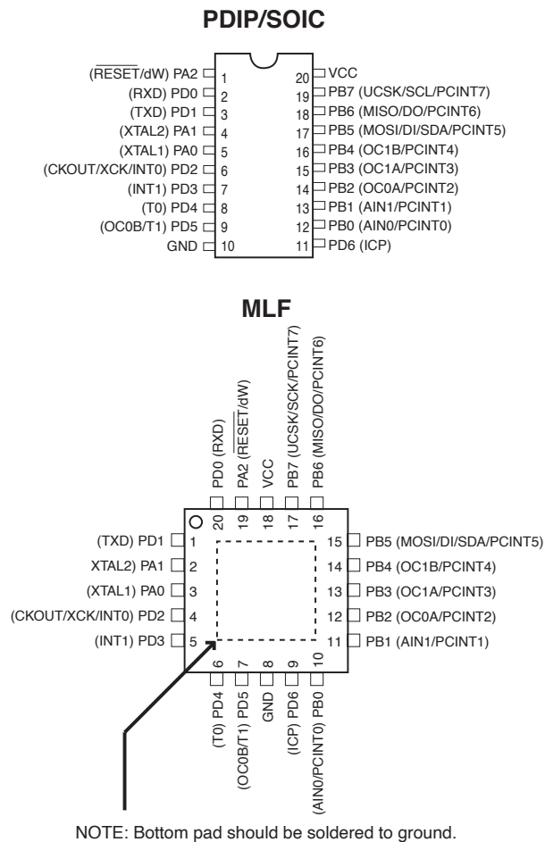
Figure 1. Pinout ATtiny2313
