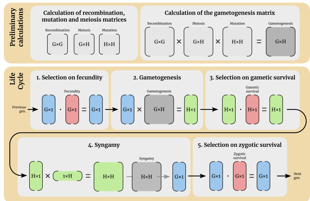
Figure 1: Summary of the various steps implemented in Ease to run simulations with a number G of genotypes and H of haplotypes. All the transition matrices (reproduction, selection, migration, ...) are available for consultation using the print method, and can be defined in a variety of ways, depending on user's requirements. Selection on gamete survival occurs simultaneously in male and female gametes, with the possibility of assigning different gamete survival rates to each sex. This also applies to selection on fertility and zygote survival when dioecious reproduction is activated.
