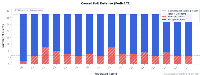
Per-Round Client Acceptance & Rejection Causal PoR (FedNEAT) vs. Baseline FedAvg + Cosine Similarity
