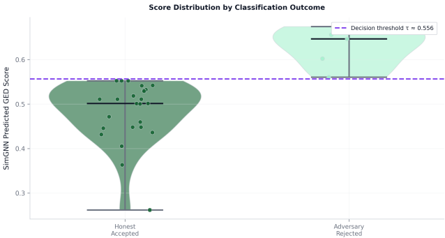
SimGNN GED Score Distribution by Client Type (Round 15) Causal PoR Defense — ASIA Dataset (N = 30 clients)
