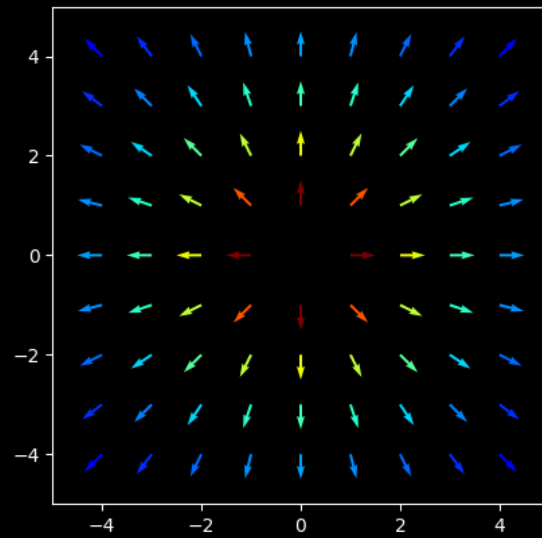
Figure 2: Sketch of the function \mathbf{v} = \frac{\hat{r}}{r^2}
