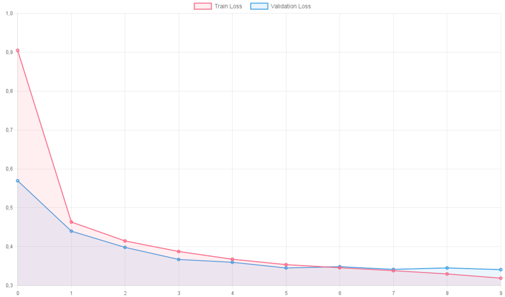
Training and Validation Loss
