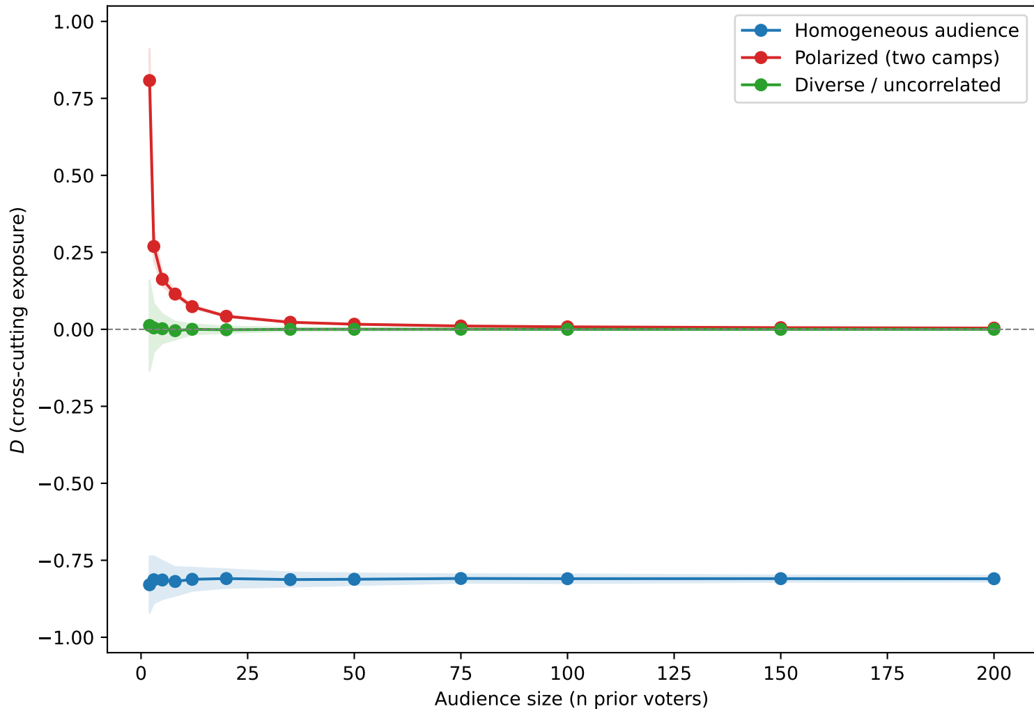
Simulated D by scenario and audience size (shaded band = \pm 1 SD across 200 Monte Carlo trials)
