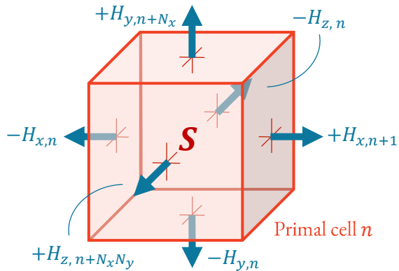
Primal Divergence Operator \mathbf{S}
