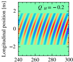
HT monitor - Bunch \Delta_H
