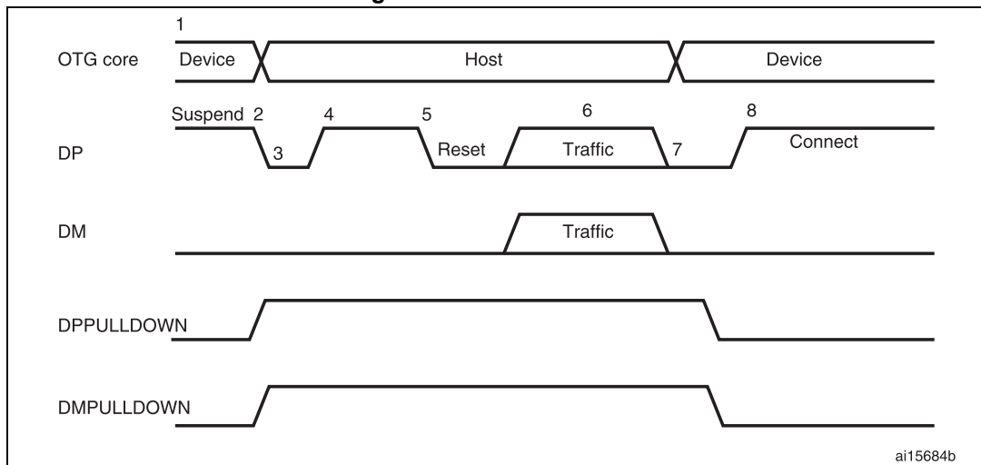
Figure 430. B-device HNP
