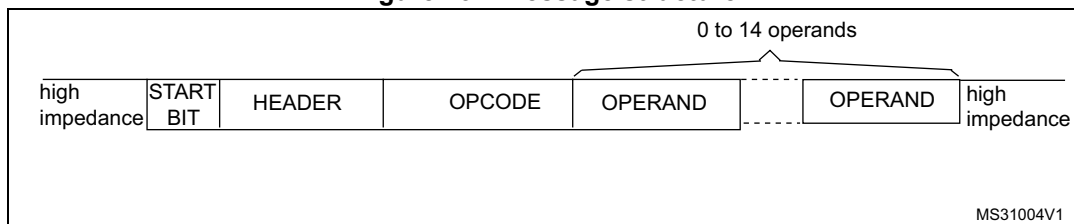
Figure 432. Message structure
