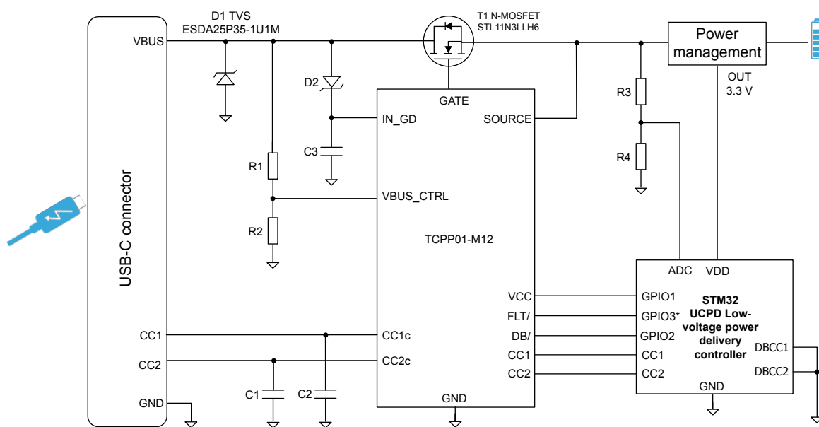
Figure 47. Sink application with battery (PD3.0)
