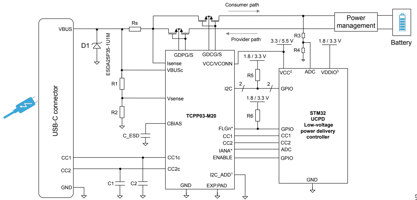
Figure 49. Battery DRP application example
