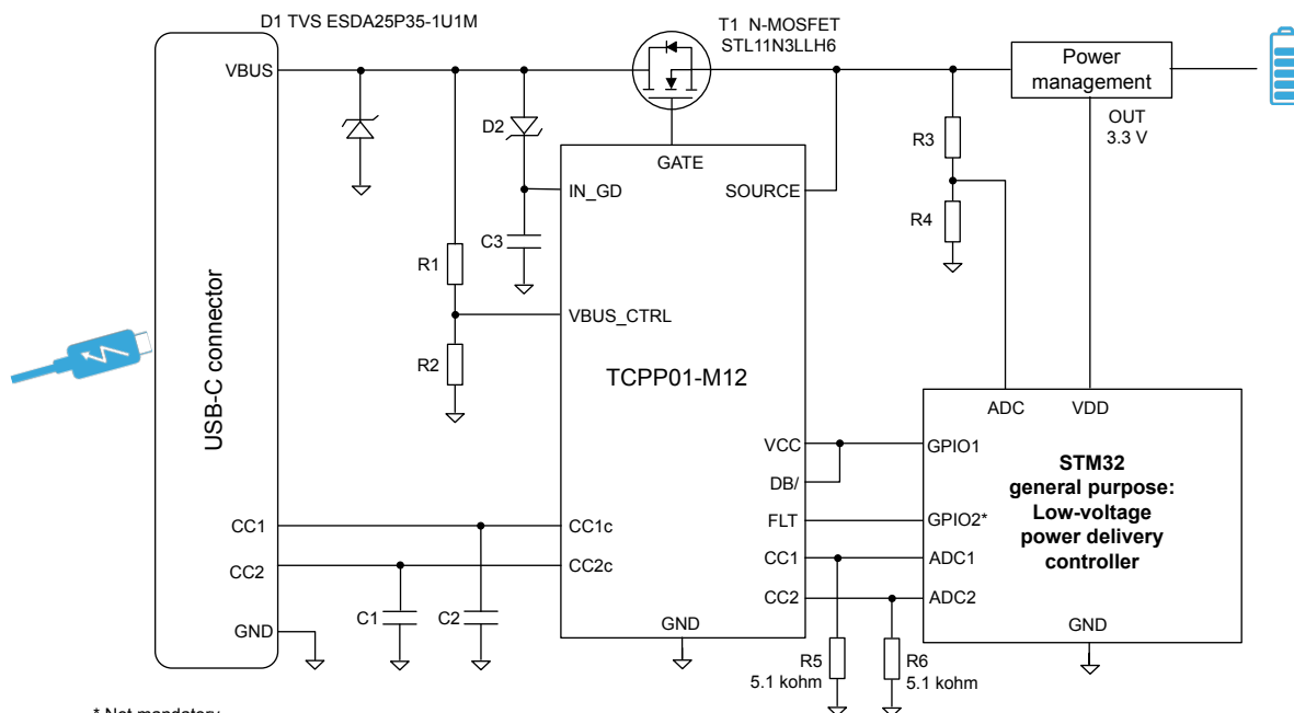
Figure 48. 15 W sink application with battery
