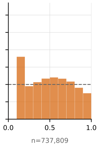
EMOS pooled
