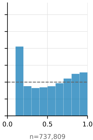
TimesFM-3 (zero-shot)
