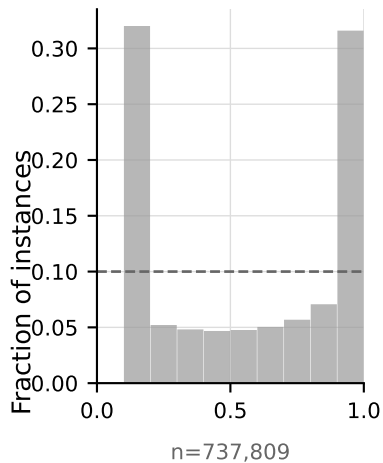
Raw ensemble
