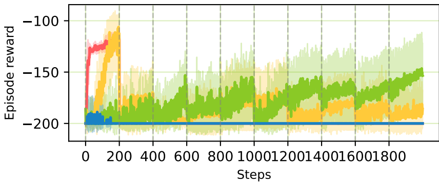
Mountaincar
