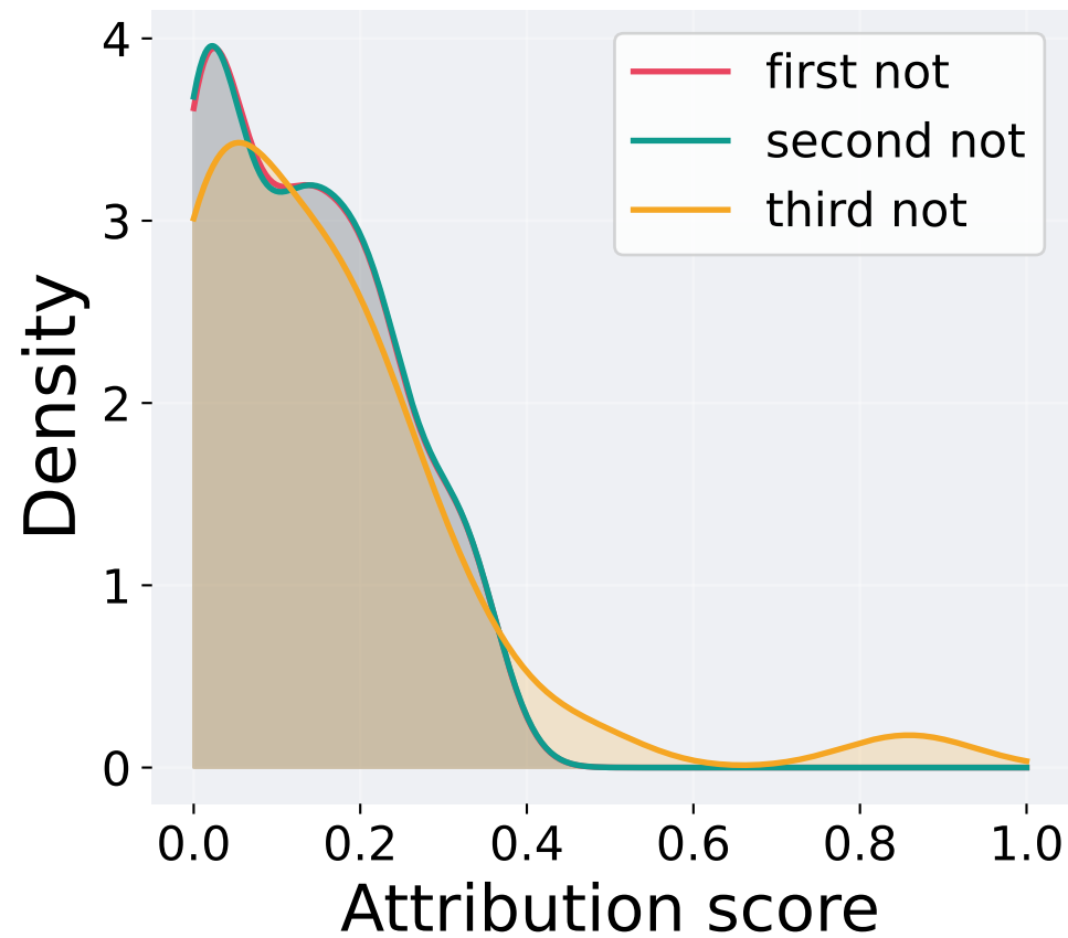
Occlusion
