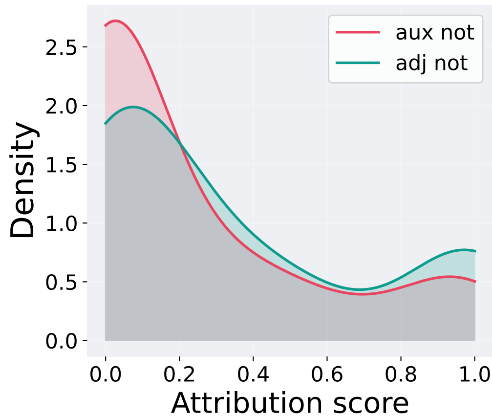
Occlusion
